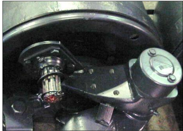
100 Series – ACB holes tapped directly into steer axle knuckle.
