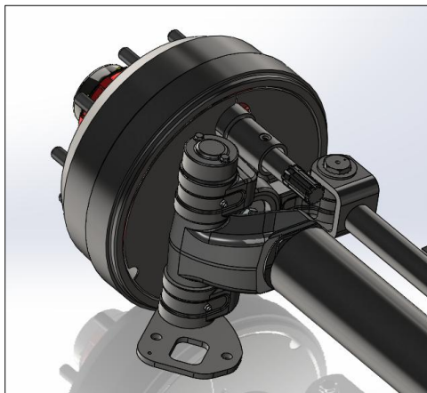
860 Series – No grease nipple in the track rod bolt
