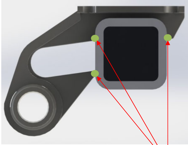
61174 Axle seat – Weld details
