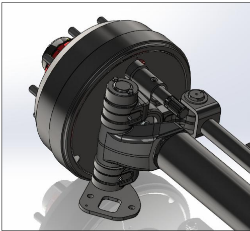
860 Series – Grease nipple shown in the track rod bolt
