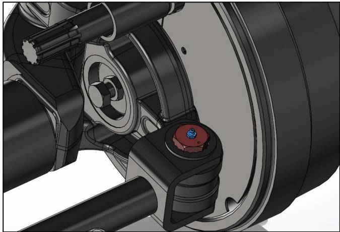
860 Series – Grease nipple shown in the track rod bolt
