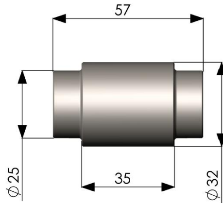
61171 – Anchor pin
