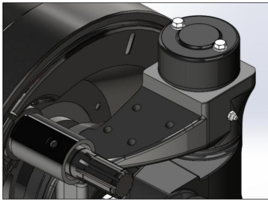
300 Series – ACB holes tapped directly into steer axle knuckle.
