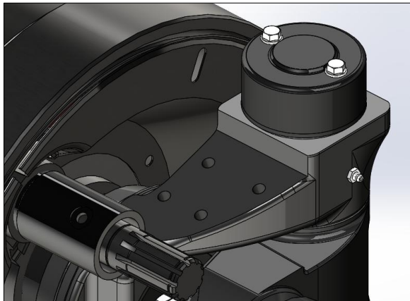
100 Series – ACB holes tapped directly into steer axle knuckle.
