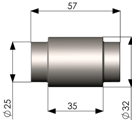
61171 – Anchor pin
